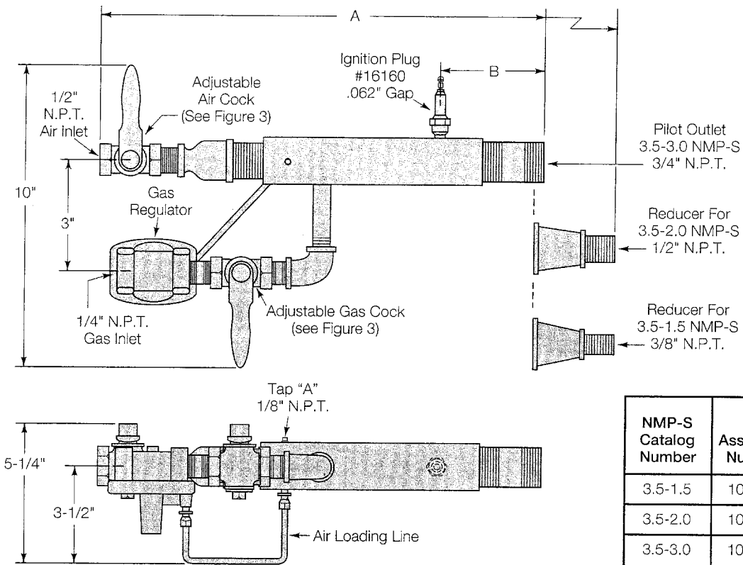
Figure 1 – 3.5 Series Capacities & Dimensions
